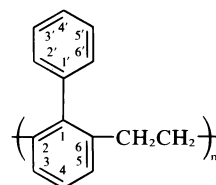
Poly(2,6-biphenyleneethylene)
