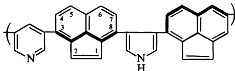
Poly(3,5-pyridinediyl-3,8-acenaphthylenylene-pyrrole-3,4-diyl-3,7-acenaphthylenylene) (heavy line denotes path followed)
