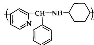
Poly(4,2-pyridinediylbenzylideneimino-1,4-cyclohexylene)
