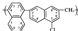
Poly[(5'-chloro-1,2'-binaphthyl-4,7'-ylene)methylene]
