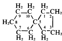
Spiro[4.5]decane
