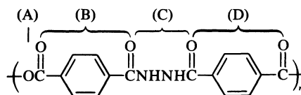
Poly(oxyterephthaloylhydrazoterephthaloyl) (not poly-(oxycarbonyl-1,4-phenylenebiscarbamoyl-1,4-phenylenecarbonyl))
