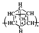
Poly(2,7-naphthylene) (not poly(7,2-naphthylene) or poly(3,6-naphthylene))
