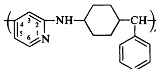
Poly(4,2-pyridinediylimino-1,4-cyclohexylenebenzylidene)
