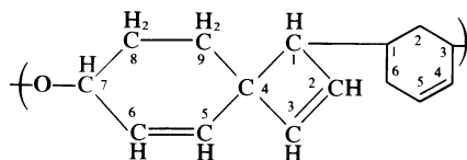
Poly(oxyspiro[3.5]nona-2,5-dien-7,1-ylene-4-cyclohexen-1,3-ylene)
