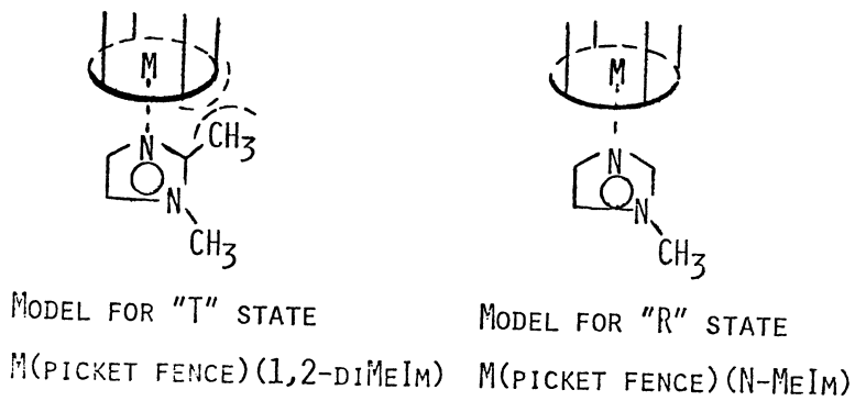
Fig. 8 Picket fence porphyrin models for Hb T and R states
