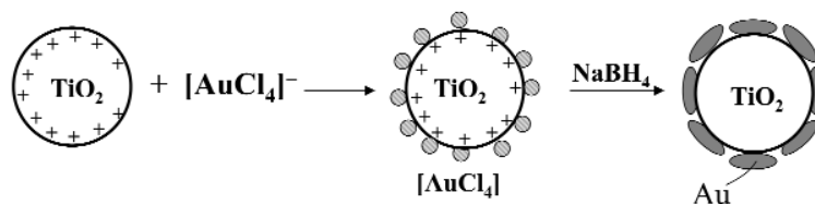
Scheme 2 Synthesis of semiconductor/metal composite colloids.
